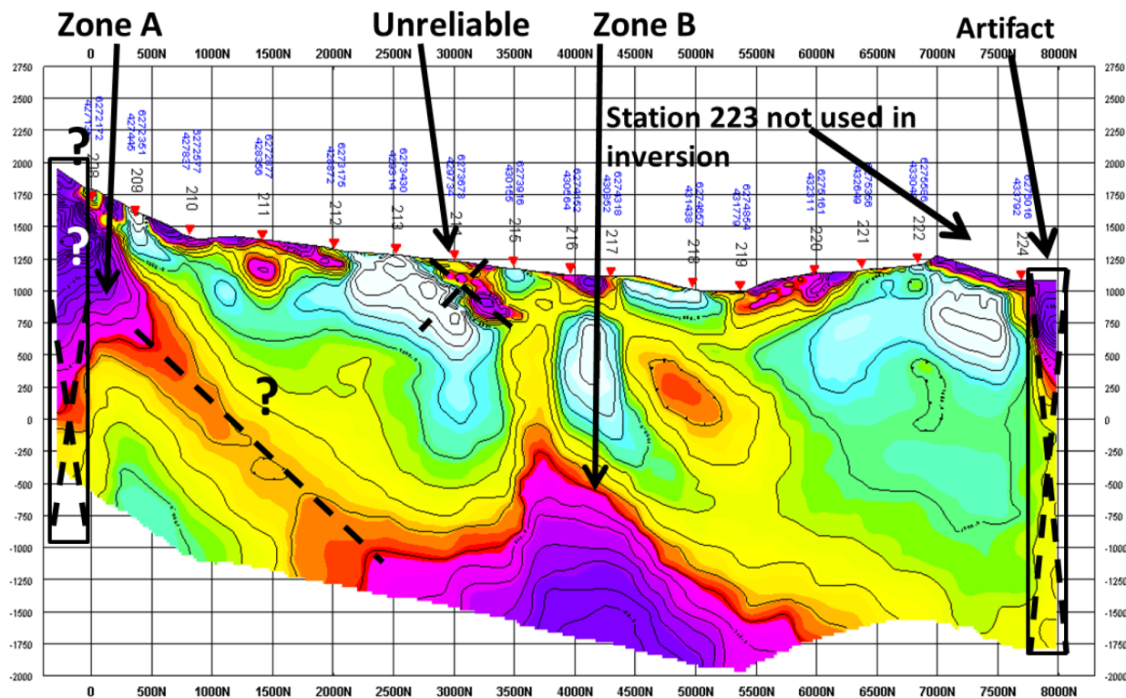
QUANTEC MAGNETOTELLURIC SURVEY OVER PART OF TREATY CREEK PROPERTY
