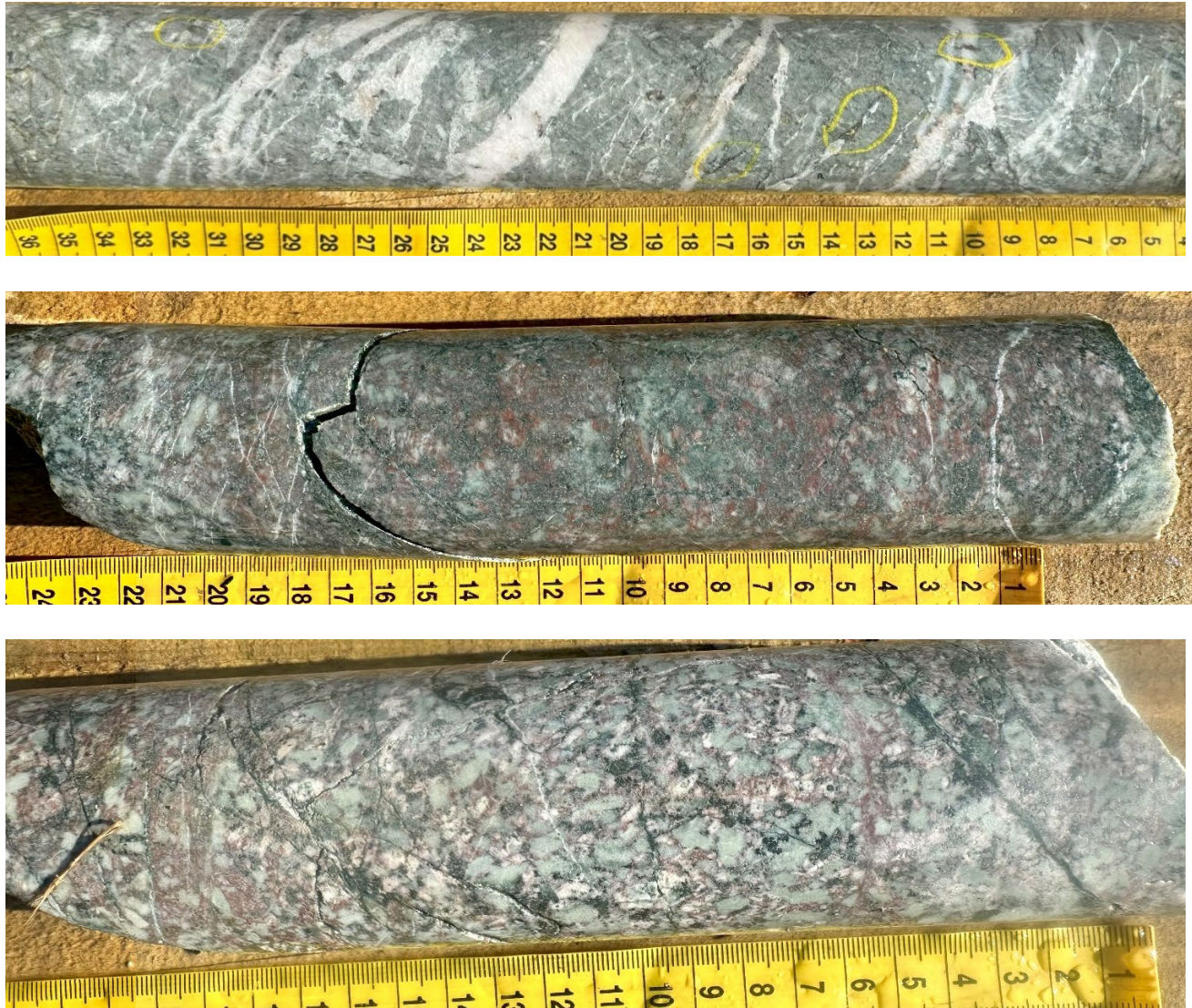
Figure 3 - Eastern Anomaly Intersections: Top: Dense quartz-calcite-chalcopryite stockwork in porphyry dyke – RAM25-02 6m. Middle: Strong K-feldspar-biotite-magnetite altered porphyry intrusion – RAM25-01 211m. Bottom: Moderately K-feldspar altered porphyry intrusion with chlorite-pyrite-chalcopryite stringers – RAM25-01 253m.
